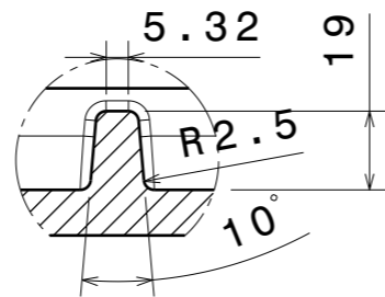
Detail view G Scale 1:2
