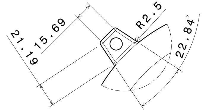
Detail view E Scale 1:2
